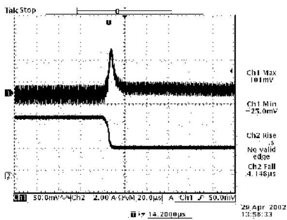
Vout=1.2V 100% to 50% load transients at 3.3V input and Ta=25° C
