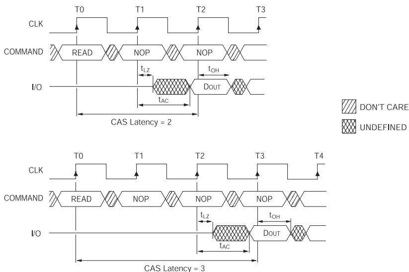
FIGURE 4 – CAS LATENCY
