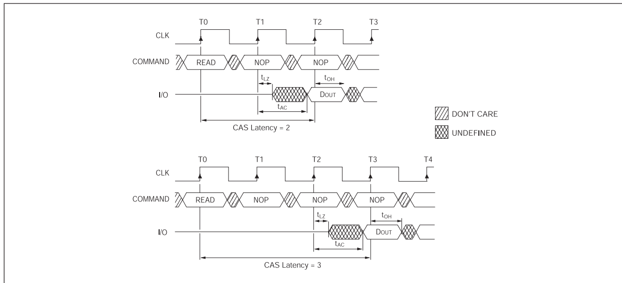
FIGURE 4 – CAS LATENCY
