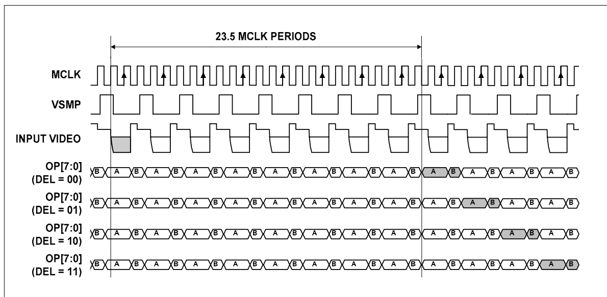
Figure 23 Mode 3 Operation
