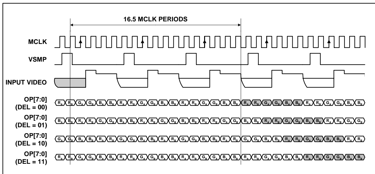
Figure 21 Mode 1 Operation
