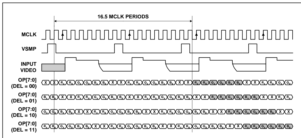
Figure 25 Mode 5 Operation (MCLK:VSMP Ratio = 8:1)
