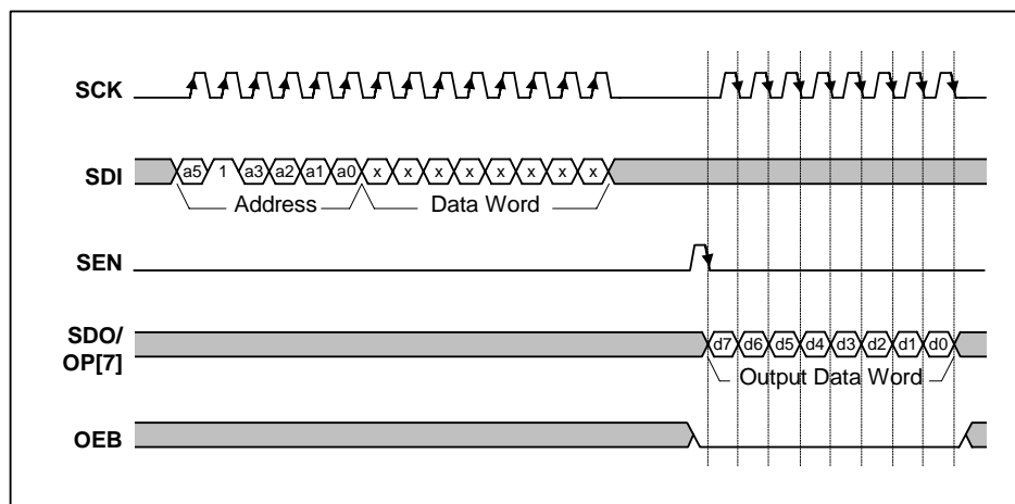
Figure 18 Serial Interface Register Read-back
