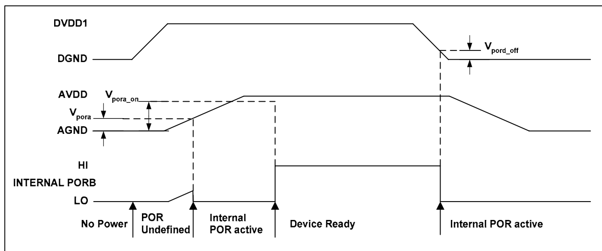
Figure 8 Typical Power up Sequence where DVDD1 is Powered before AVDD
