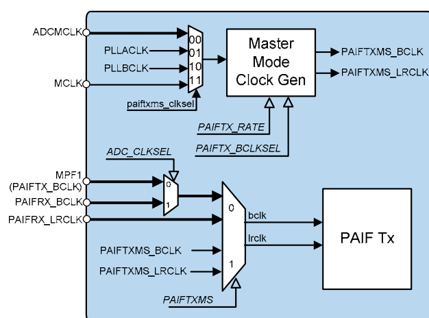
Figure 30 PAIF Transmitter Clock Selection
