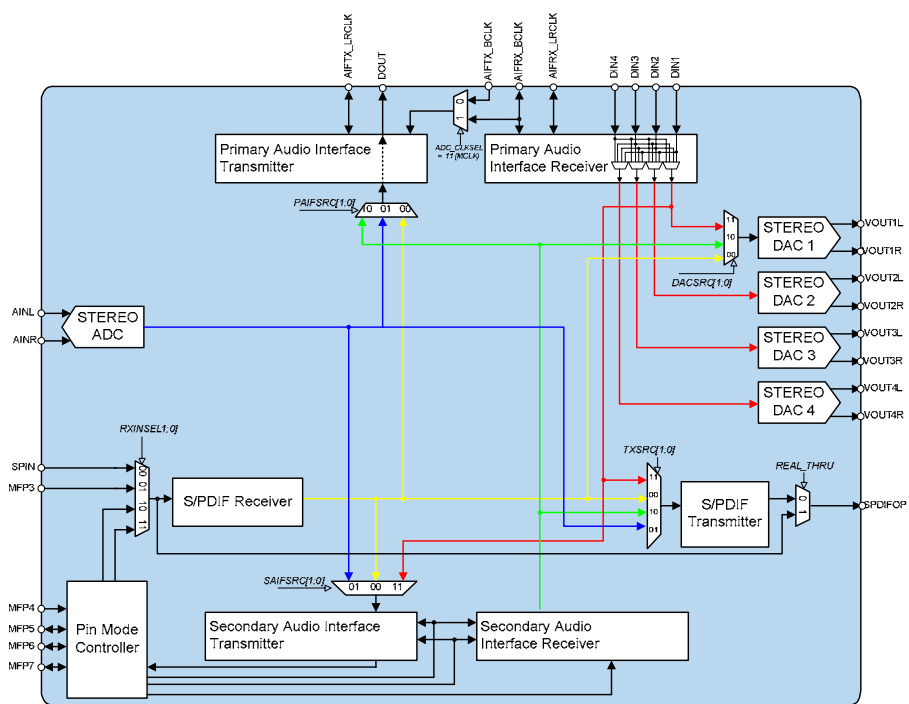
Figure 25 Digital Routing
