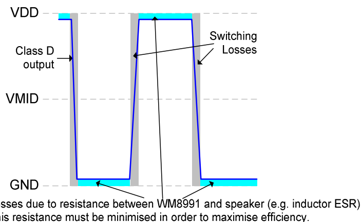
Figure 105 Speaker Connection Losses
