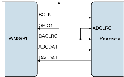
Figure 53 Master Mode with ADCLRC as GPIO
