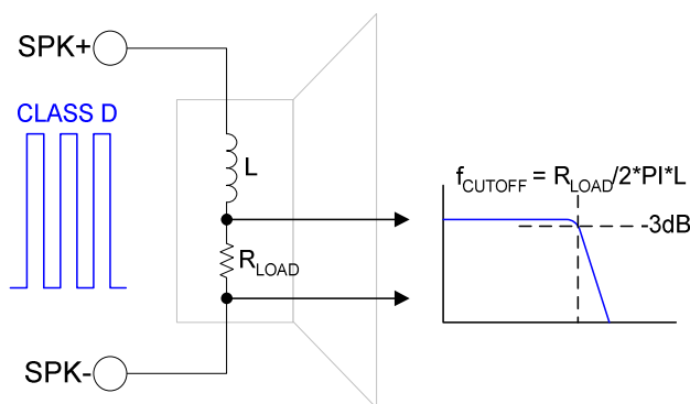
Figure 104 Speaker Equivalent Circuit
