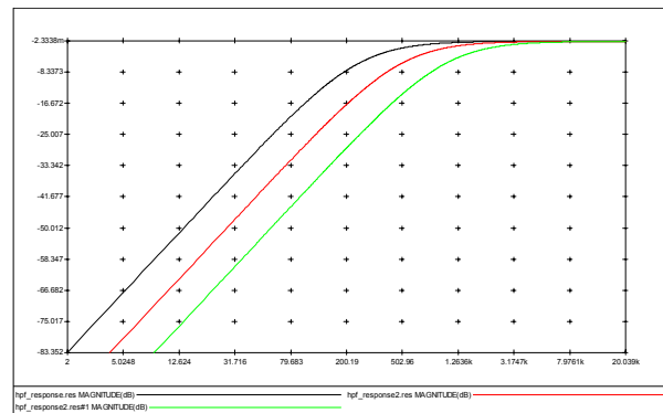
Figure 93 ADC Digital High Pass Filter Ripple (48kHz, Voice Mode, ADC_HPF_CUT=01, 10 and 11)
