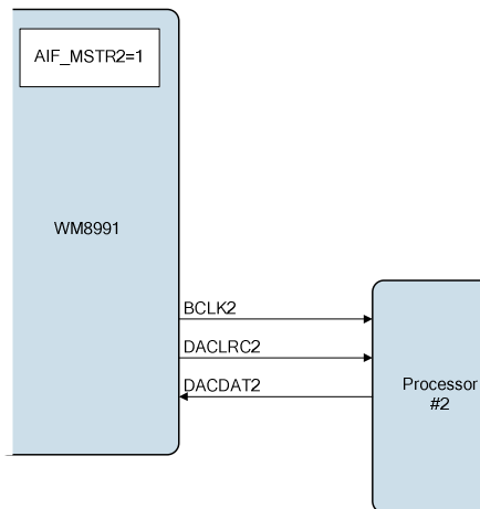
Figure 55 Interface 2 = Master
