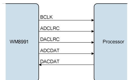
Figure 51 Master Mode
