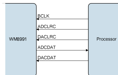
Figure 52 Slave Mode
