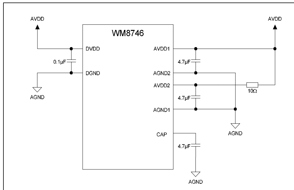
Figure 26 Decoupling Example 2
