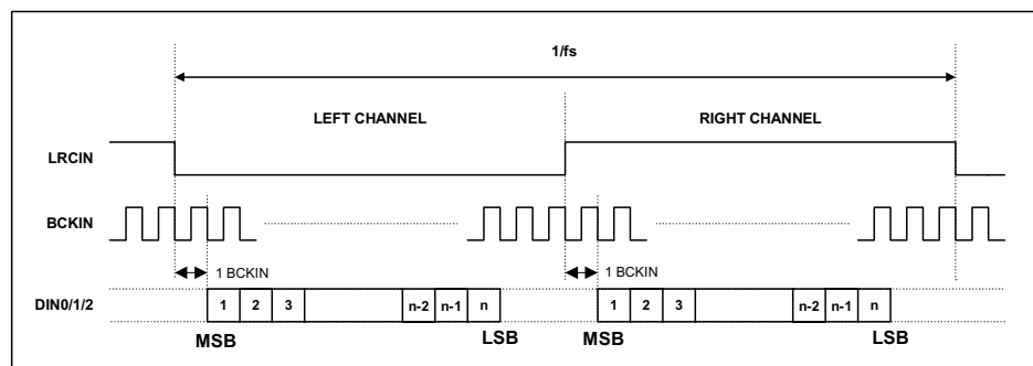
Figure 6 I 2 S Mode Timing Diagram
