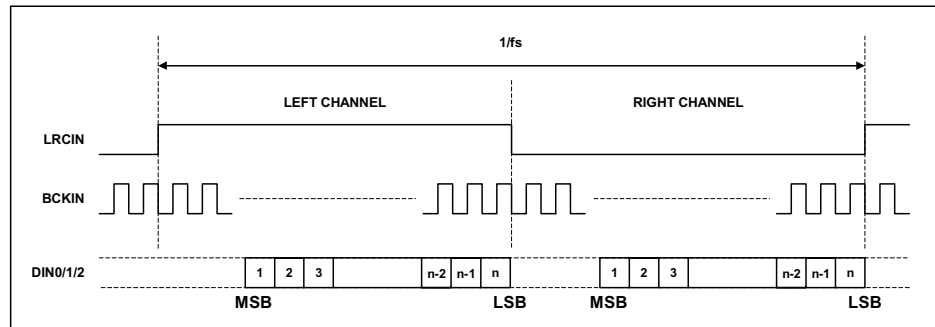
Figure 5 Right Justified Mode Timing Diagram
