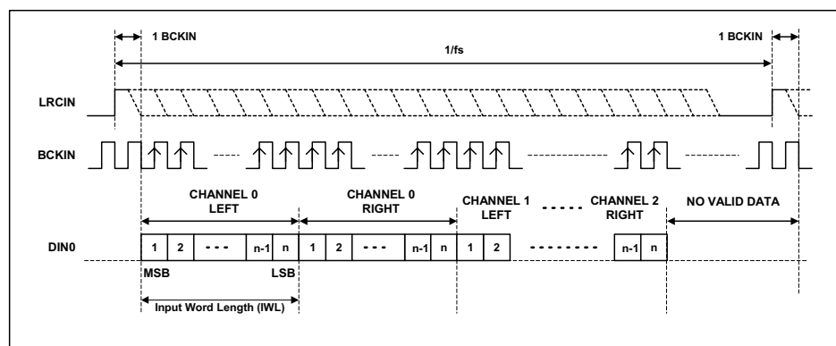
Figure 7 DSP Mode A Timing Diagram
