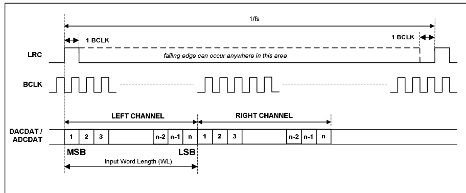
Figure 23 DSP/PCM Mode Audio Interface (mode B, LRP=0, Slave)
