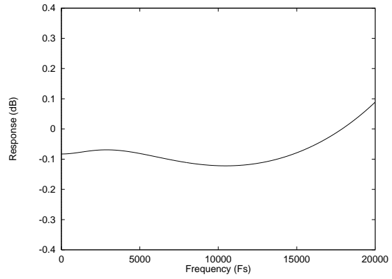
Figure 46 De-emphasis Error (44.1kHz)
