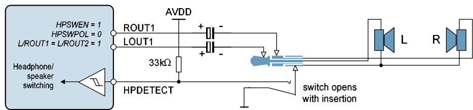
Figure 11 Example Headset Detection Circuit Using Normally-Open Switch
