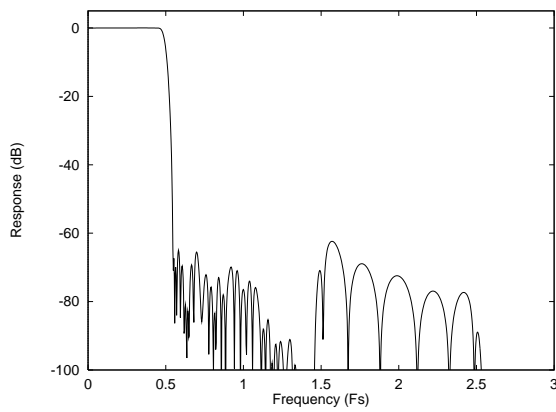
Figure 35 ADC Digital Filter Frequency Response – Type 0
