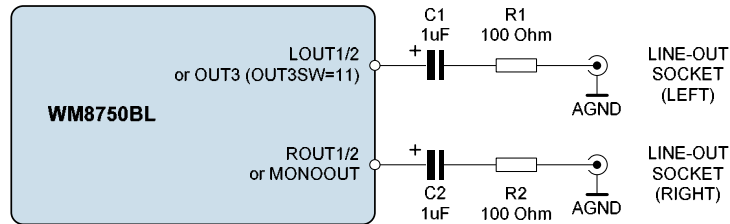
Figure 15 Recommended Circuit for Line Output
