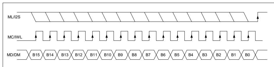
Figure 34 3-Wire SPI Compatible Interface
