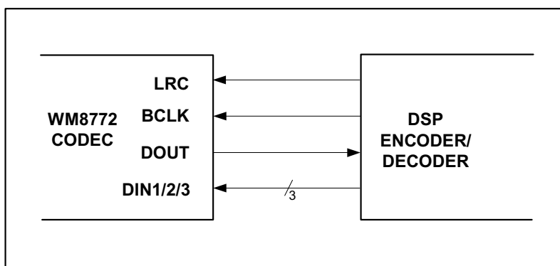
Figure 21 Slave Mode
