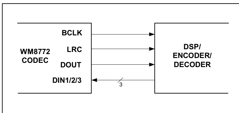
Figure 22 Master Mode
