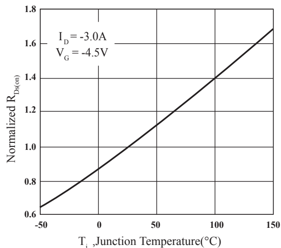
Fig.4 Normalized On-Resistance
