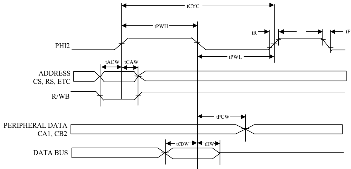
Figure 3-2 Read Timing
