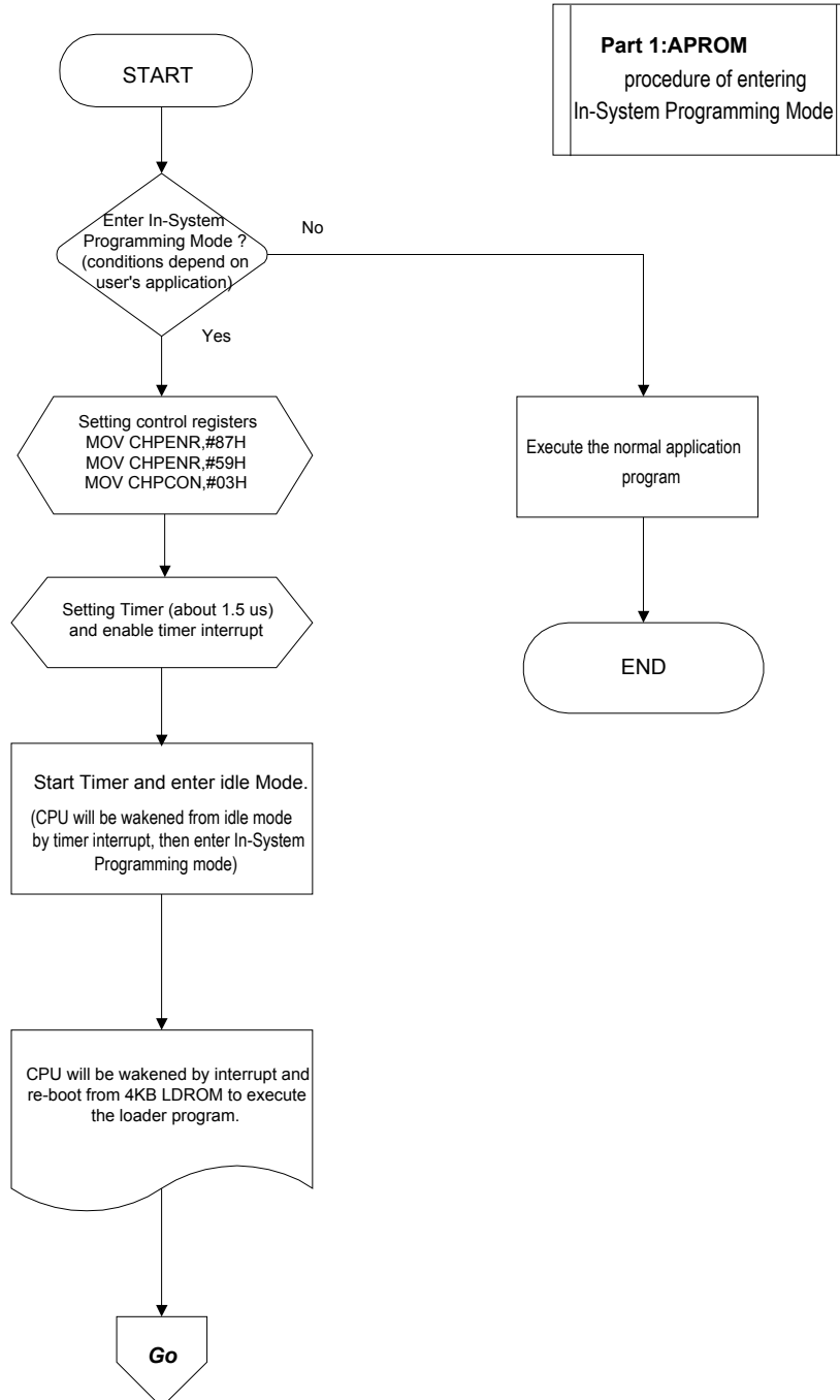
Figure 15-1 The algorithm of ISP for AP ROM
