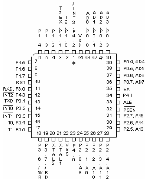
44-Pin PLCC
