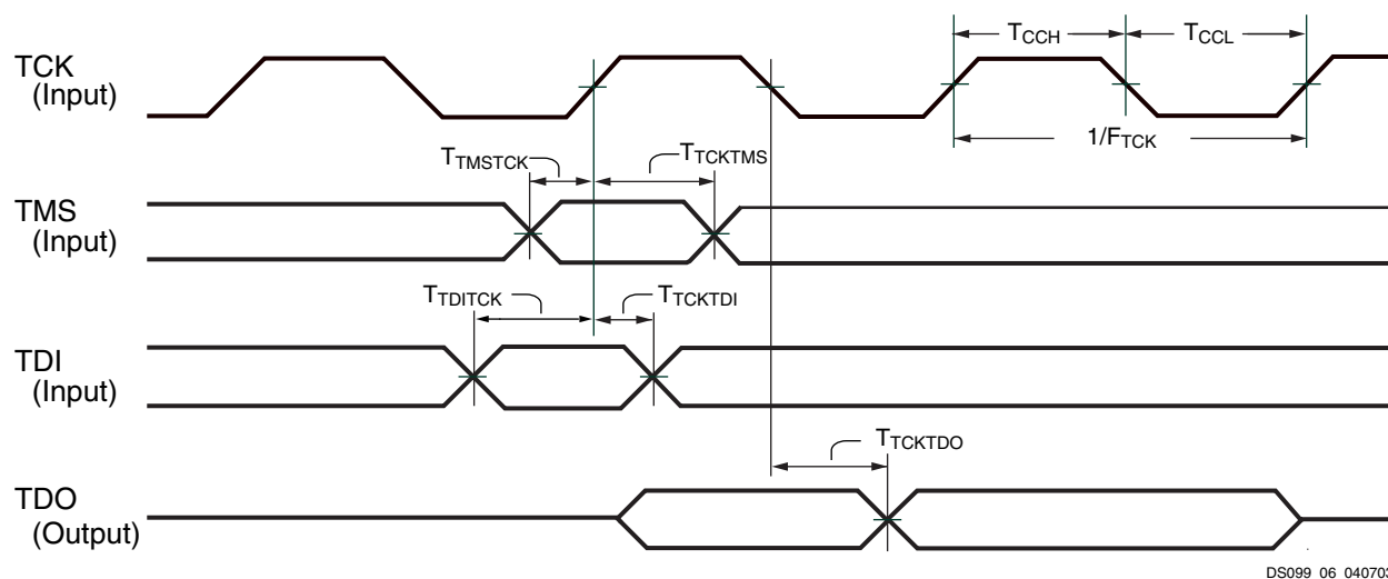
Figure 8: JTAG Waveforms
