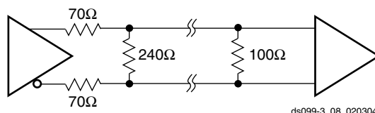
Figure 3: External Terminations for LVPECL
