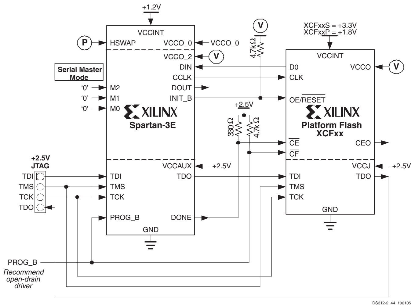
Figure 51: Master Serial Mode using Platform Flash PROM
