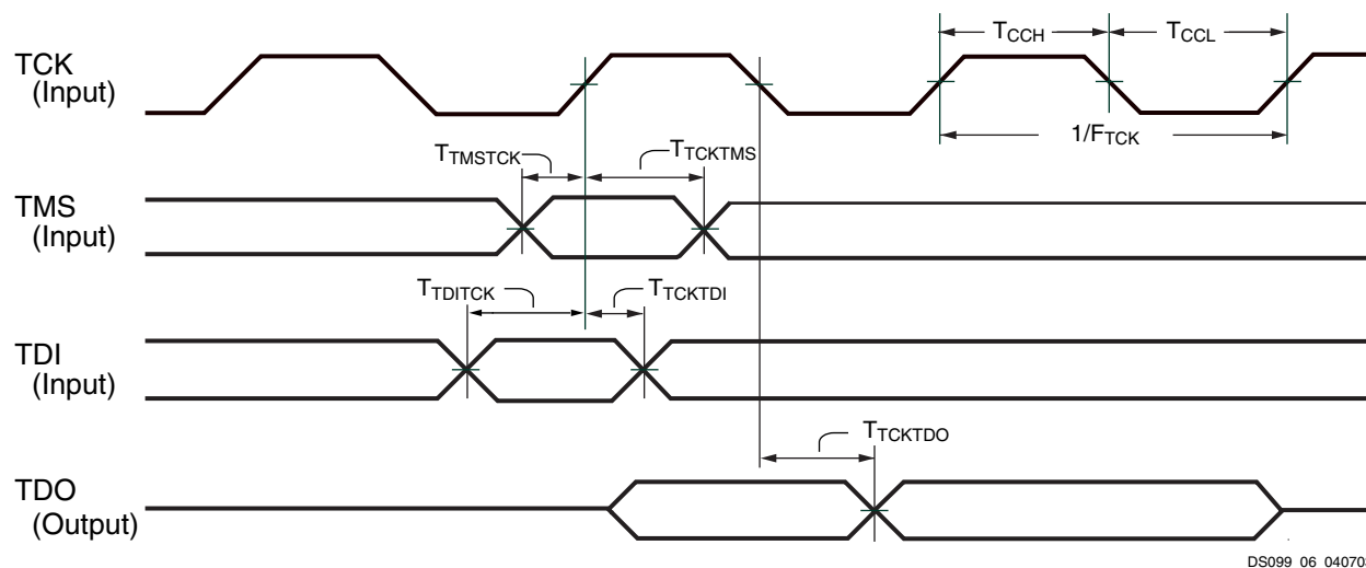
Figure 79: JTAG Waveforms
