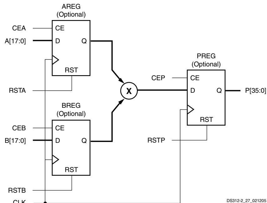
Figure 36: Principle Ports and Functions of Dedicated Multiplier Blocks
