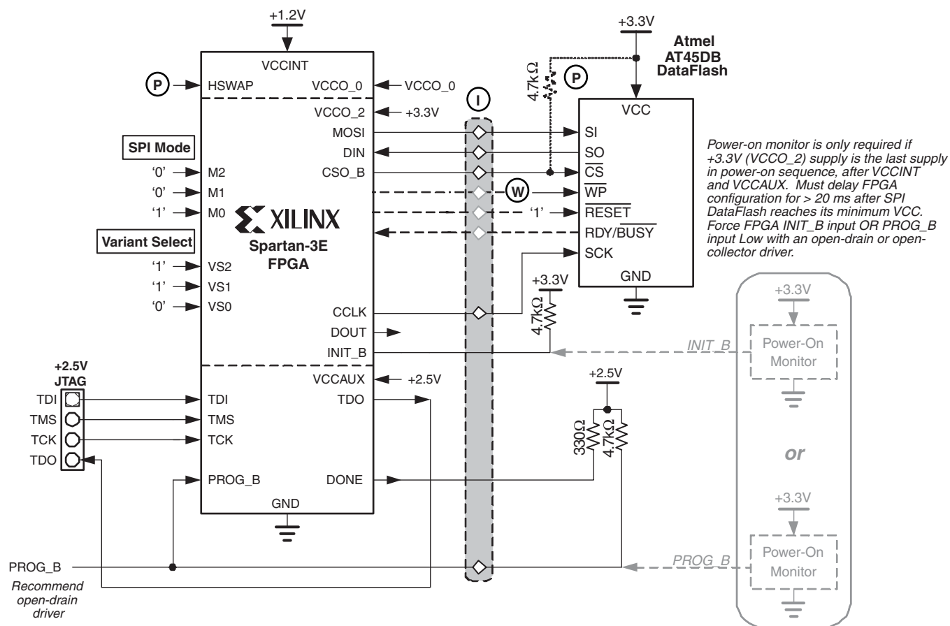
Figure 54: Atmel SPI-based DataFlash Configuration Interface
