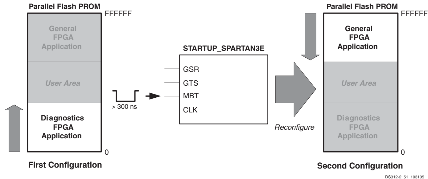
Figure 60: Use MultiBoot to Load Alternate Configuration Images
