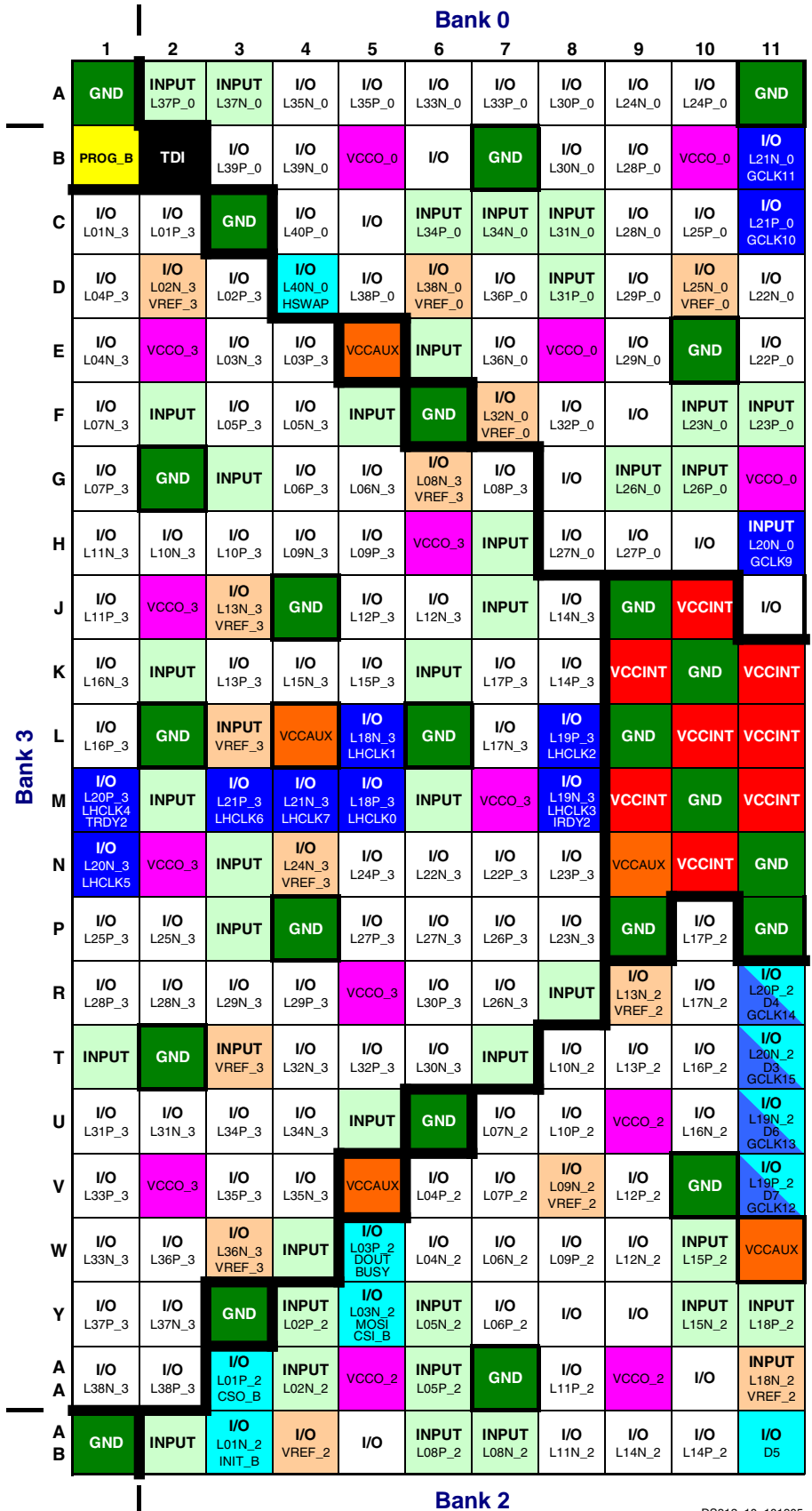
Figure 89: FG484 Package Footprint (top view)
