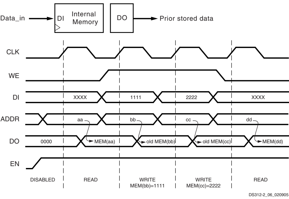
Figure 34: Waveforms of Block RAM Data Operations with READ_FIRST Selected
