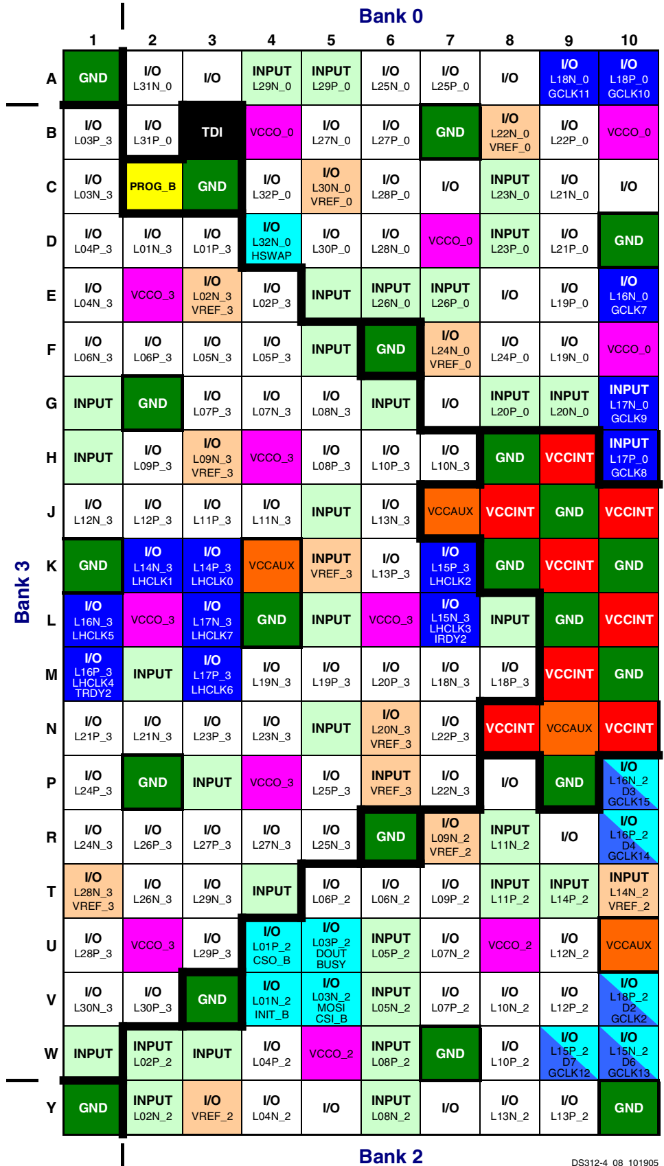
Figure 88: FG400 Package Footprint (top view)
