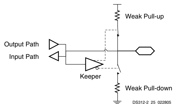
Figure 12: Keeper Circuit
