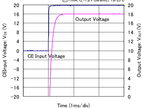
XC6701B J02
