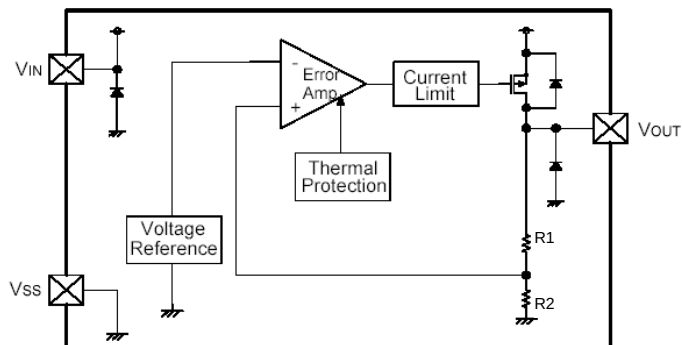
●XC6701D Series (SOT-89, SOT-223, TO-252)
