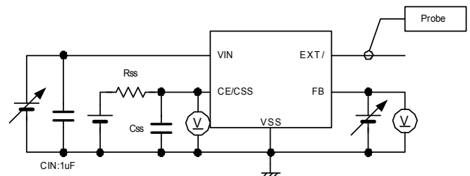
Circuit 5: Soft-Start (Externally set: B and D series)
