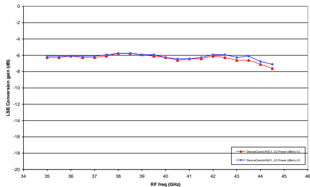
XM1000-BD: LSB Conversion gain (dB) vs. RF freq (GHz) Vg = -1.1V, LO = 12dBm, IF = 1GHz
