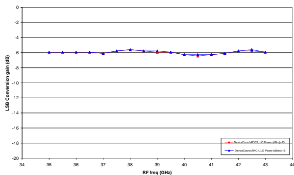
XM1000-BD: LSB Conversion gain (dB) vs. RF freq (GHz) Vg = -1.1V, LO = 15dBm, IF = 1GHz
