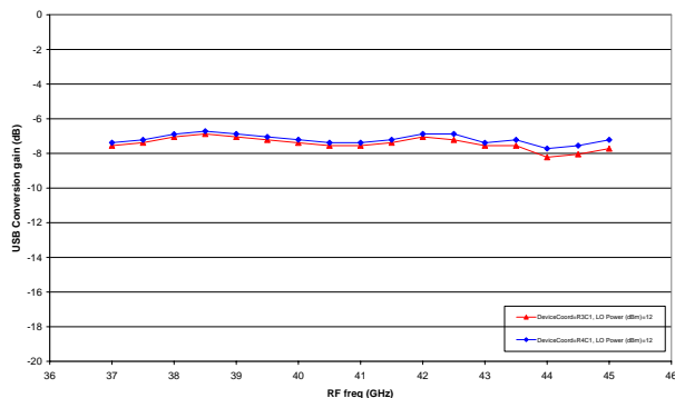
XM1000-BD: USB Conversion gain (dB) vs. RF freq (GHz) Vg = -1.1V, LO = 12dBm, IF = 3GHz
