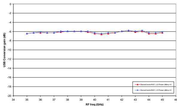
XM1000-BD: USB Conversion gain (dB) vs. RF freq (GHz) Vg = -1.1V, LO = 12dBm, IF = 1GHz
