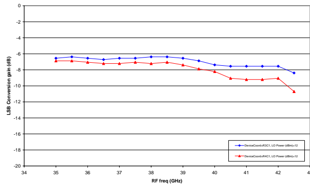
XM1000-BD: LSB Conversion gain (dB) vs. RF freq (GHz) Vg = -1.1V, LO = 12dBm, IF = 3GHz
