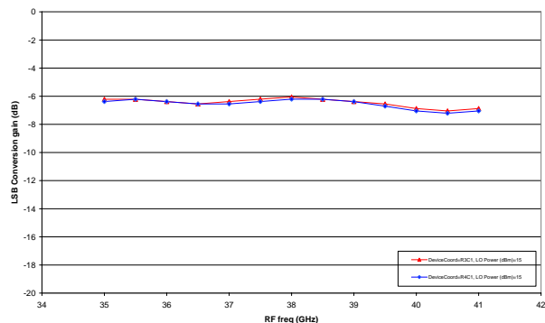
XM1000-BD: LSB Conversion gain (dB) vs. RF freq (GHz) Vg = -1.1V, LO = 15dBm, IF = 3GHz
