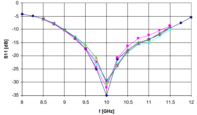
Input return loss ( V_d=8V , V_{gg}=-5V , P_s=17dBm )
