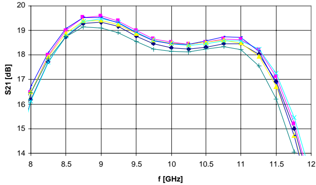
Small signal Gain ( V_d=8V , V_{gg}=-5V , P_s=-20dBm )
