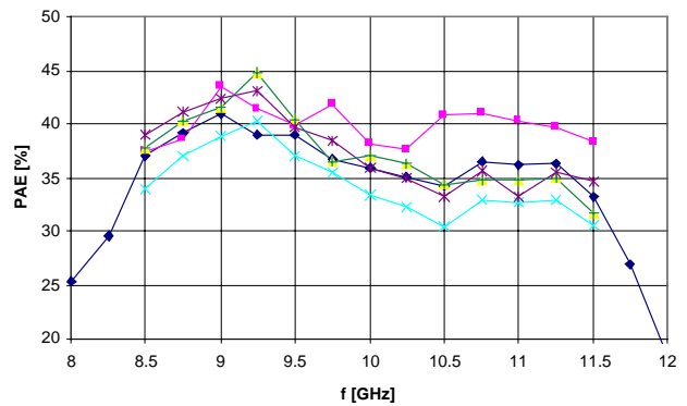
Power Added Efficiency ( V_d=8V , V_{gg}=-5V , P_s=17dBm )
