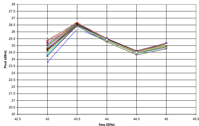
0470_wafer sweep: Pout vs Freq at Pin = 14dBm
