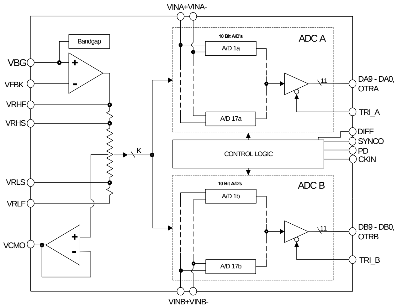
Figure 1. XRD64L43 Simplified Block Diagram
