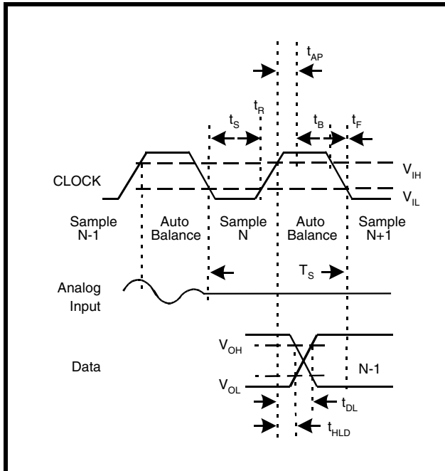
FIGURE 3. XRD87L99 TIMING DIAGRAM
