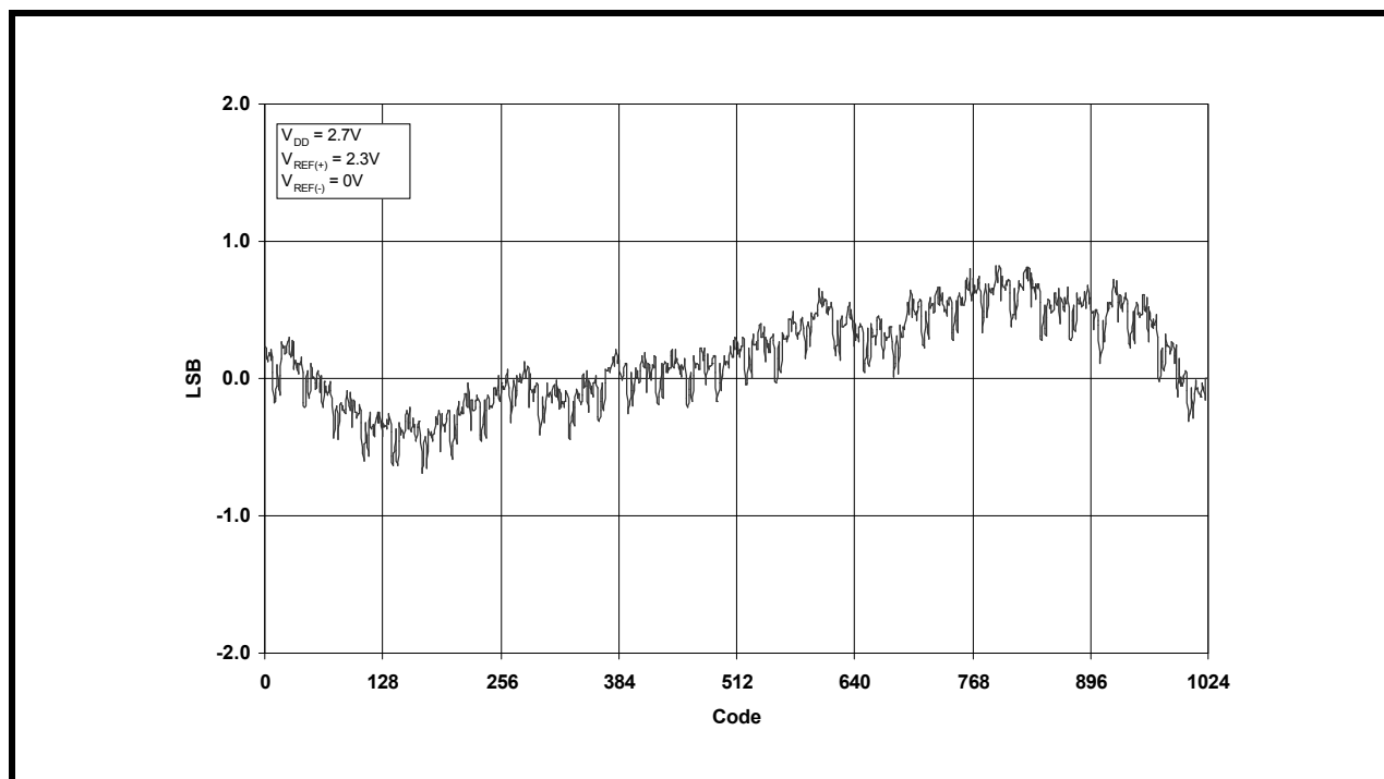
FIGURE 30. INL @ 2MSPS
