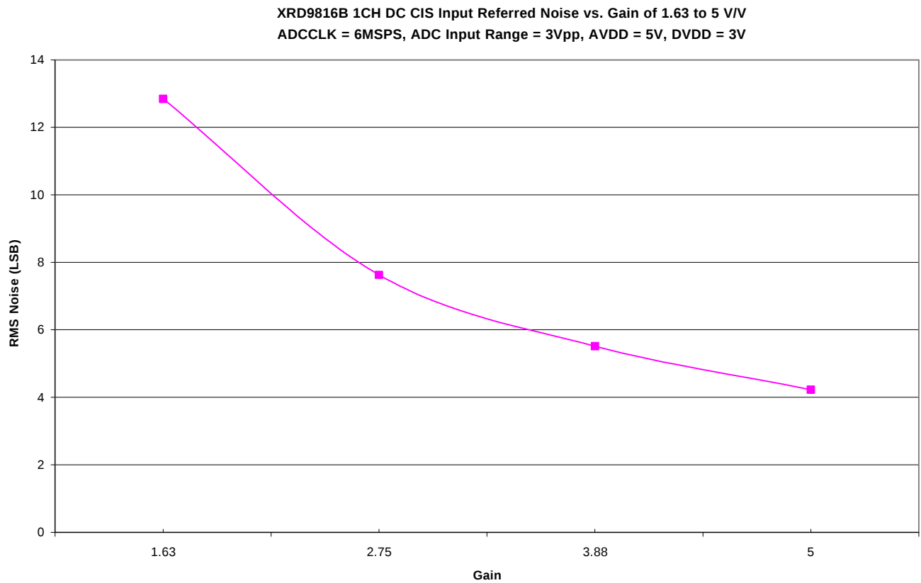
Graph 11. XRD9816B 1-Channel CIS SS/H No Clamp Input Referred Noise vs. Gain (6 MSPS)
