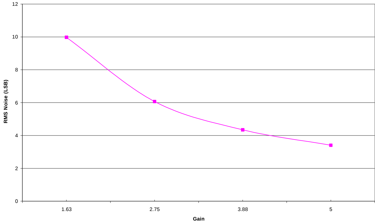
Graph 10. XRD9816B 1-Channel CIS SS/H No Clamp Input Referred Noise vs. Gain (1 MSPS)
