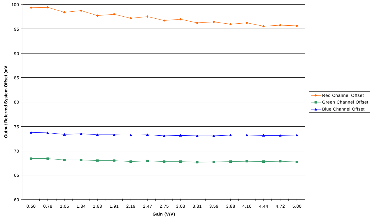
Graph 8. XRD9814B /9816B 3-Channel CDS Pixel Clamp System Offset vs. Gain
