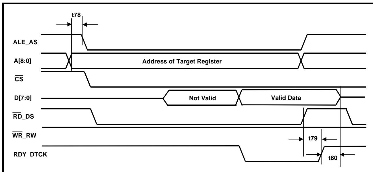
FIGURE 18. MICROPROCESSOR INTERFACE TIMING—MOTOROLA TYPE PROCESSORS (READ OPERATIONS) NON-BURST MODE
