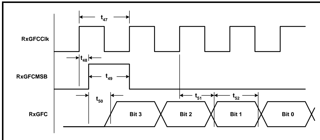
FIGURE 14. GFC NIBBLE-FIELD SERIAL OUTPUT PORT TIMING (RECEIVE CELL PROCESSOR)
