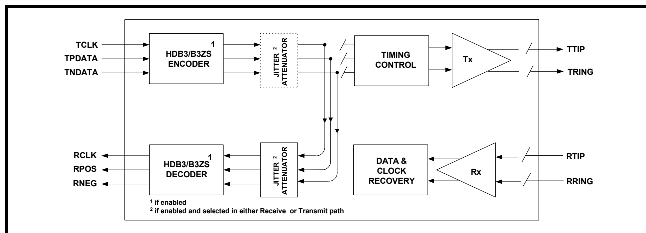
FIGURE 26. DIGITAL LOOPBACK
