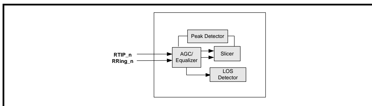
FIGURE 7. ACG/EQUALIZER BLOCK DIAGRAM
