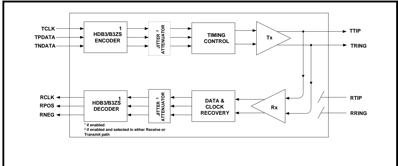
FIGURE 26. ANALOG LOOPBACK
