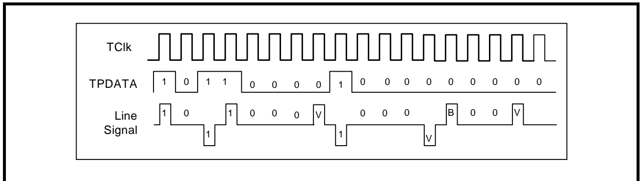
FIGURE 15. HDB3 ENCODING FORMAT
