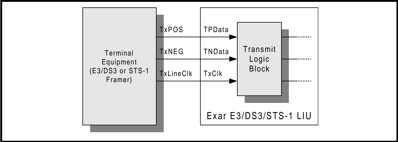
FIGURE 3. TYPICAL INTERFACE BETWEEN TERMINAL EQUIPMENT AND THE XRT75L04D (DUAL-RAIL DATA)
