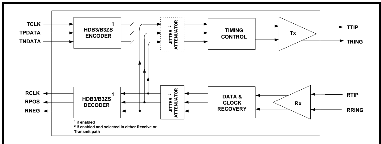
FIGURE 29. REMOTE LOOPBACK
