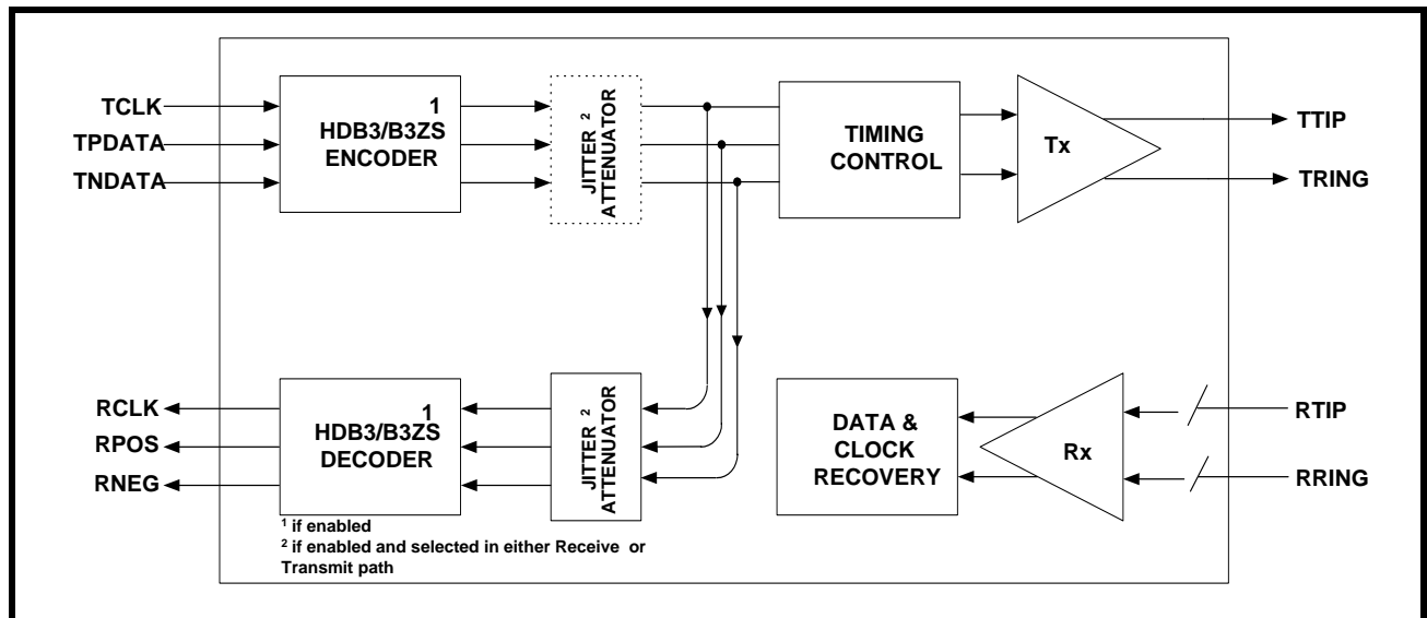
FIGURE 28. DIGITAL LOOPBACK
