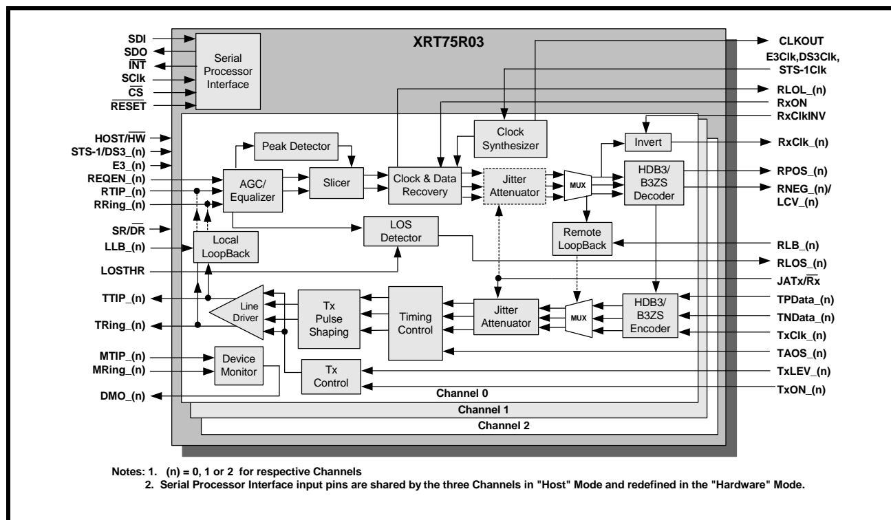
FIGURE 1. BLOCK DIAGRAM OF THE XRT 75R03
