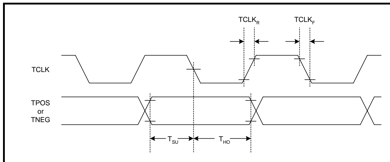
FIGURE 16. TRANSMIT DATA SAMPLED ON FALLING EDGE OF TCLK
