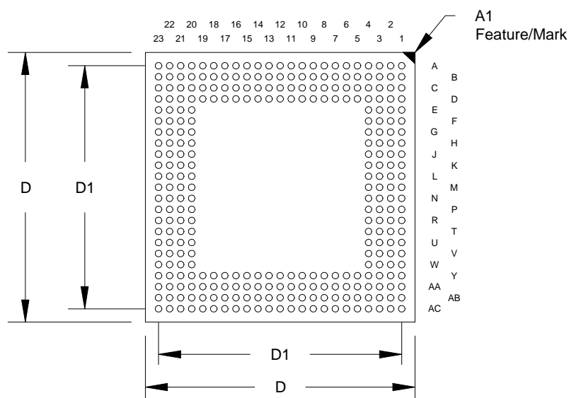
304 Ball Plastic Ball Grid Array (31.0 mm x 31.0 mm, 1.27mm pitch PBGA)
