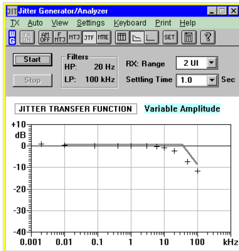
FIGURE 45. JITTER TRANSFER FUNCTION - JA DISABLED
