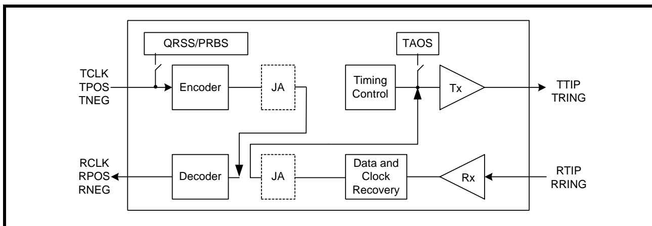
FIGURE 25. SIMPLIFIED BLOCK DIAGRAM OF DUAL LOOPBACK
