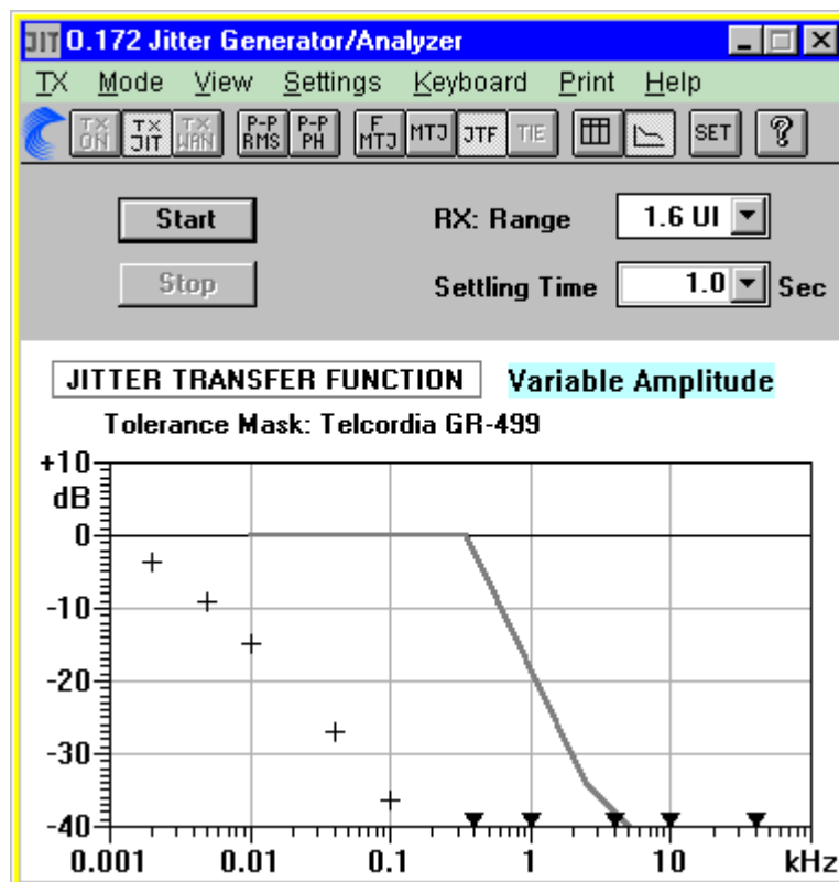
FIGURE 41. JITTER TRANSFER FUNCTION - T1 RX 3Hz 64BITS
