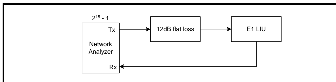
FIGURE 42. TEST CIRCUIT FOR E1 JITTER TOLERANCE
