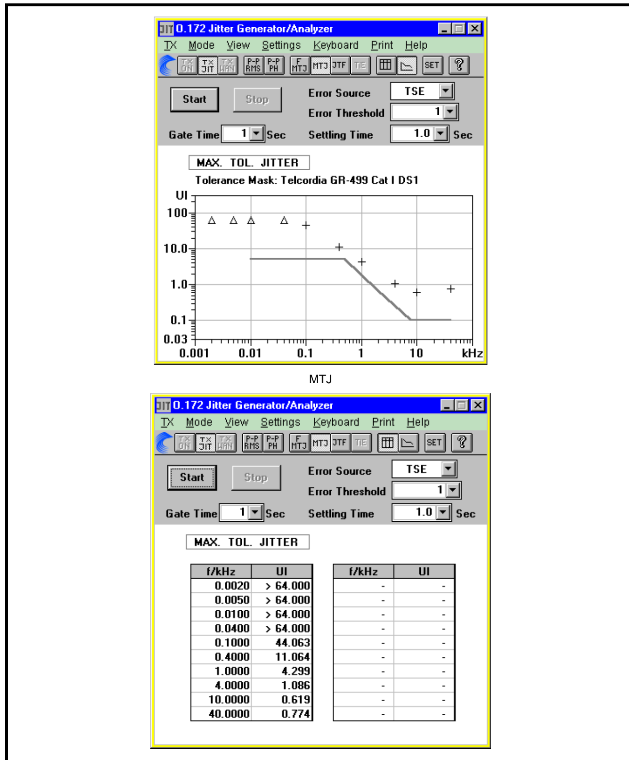
FIGURE 36. DS-1 JITTER TOLERANCE
