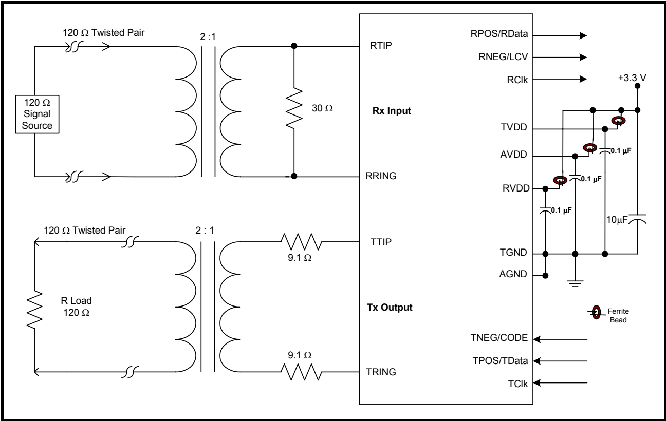
FIGURE 19. INTERFACING THE XRT83L216 TO THE LINE FOR 120 \Omega APPLICATIONS (1CHANNEL SHOWN)
