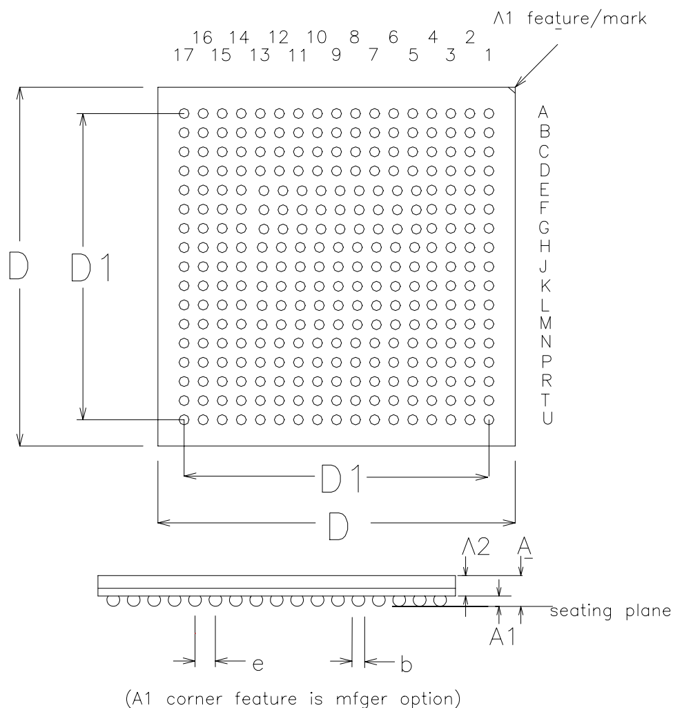
FIGURE 21. 15x15MM 289 BALL STBGA
