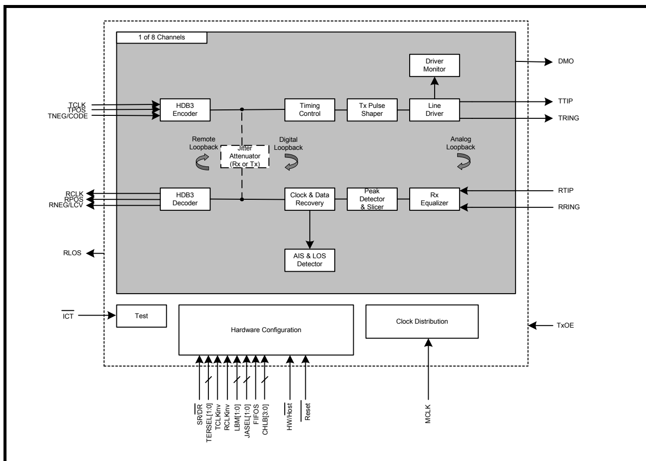
FIGURE 2. HARDWARE MODE BLOCK DIAGRAM OF THE XRT83SL28
