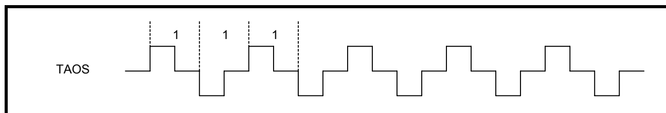
FIGURE 15. TAOS (TRANSMIT ALL ONES)ATAOS (AUTOMATIC TRANSMIT ALL ONES)
