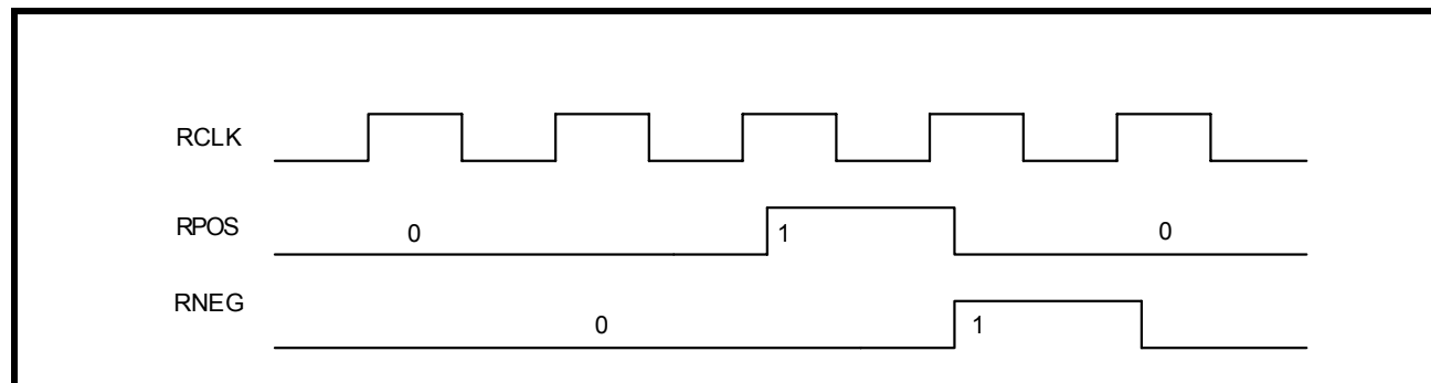
FIGURE 11. DUAL RAIL MODE WITH A FIXED REPEATING "0011" PATTERN
