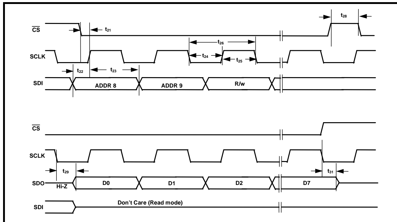
FIGURE 37. TIMING DIAGRAM FOR THE MICROPROCESSOR SERIAL INTERFACE
