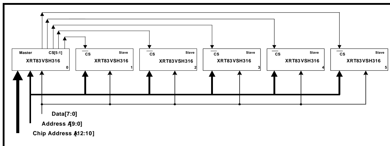
FIGURE 27. SIMPLIFIED BLOCK DIAGRAM OF AN 84-CHANNEL APPLICATION
