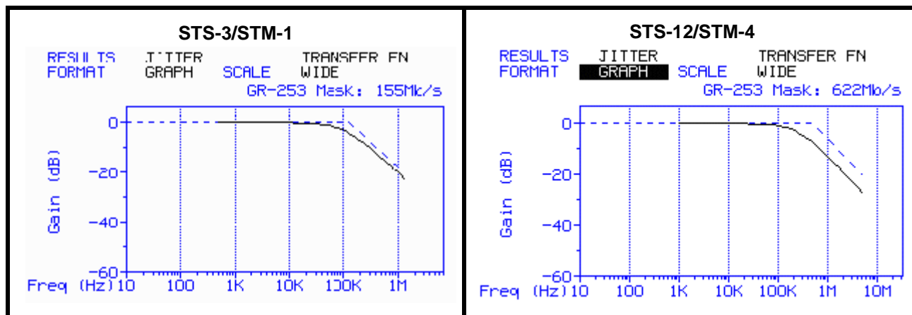
FIGURE 26. XRT91L31 MEASURED JITTER TRANSFER WITH 77.76MHz REFERENCE CLOCK
