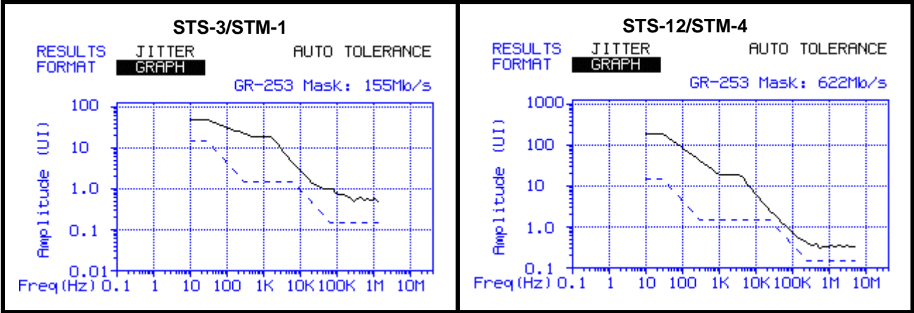
FIGURE 24. XRT91L31 MEASURED JITTER TOLERANCE WITH 77.76MHz REFERENCE CLOCK
