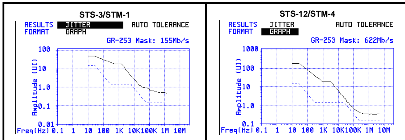
FIGURE 25. XRT91L31 MEASURED JITTER TOLERANCE WITH 19.44MHz REFERENCE CLOCK
