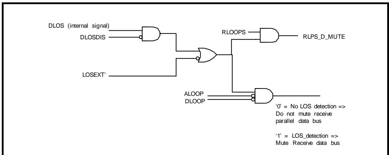
FIGURE 7. LOS DECLARATION CIRCUIT
