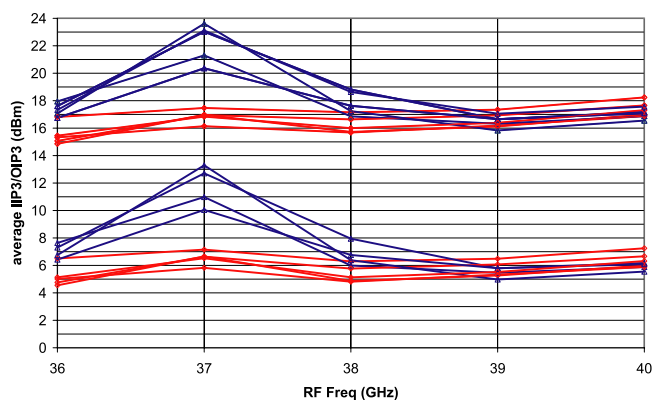
XR1004-BD (USB, IF = 2 GHz, Pout_scl = -9 dBm): aver OIP3 vs RF LO = -2 dBm (red) and +2 dBm (blue), 5 devices measured
