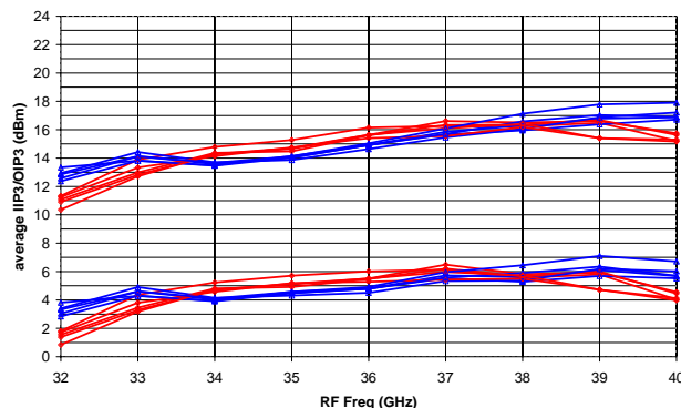
XR1004-BD (LSB, IF = 2 GHz, Pout_scl = -9 dBm): aver OIP3 vs RF LO = -2 dBm (red) and +2 dBm (blue), 5 devices measured
