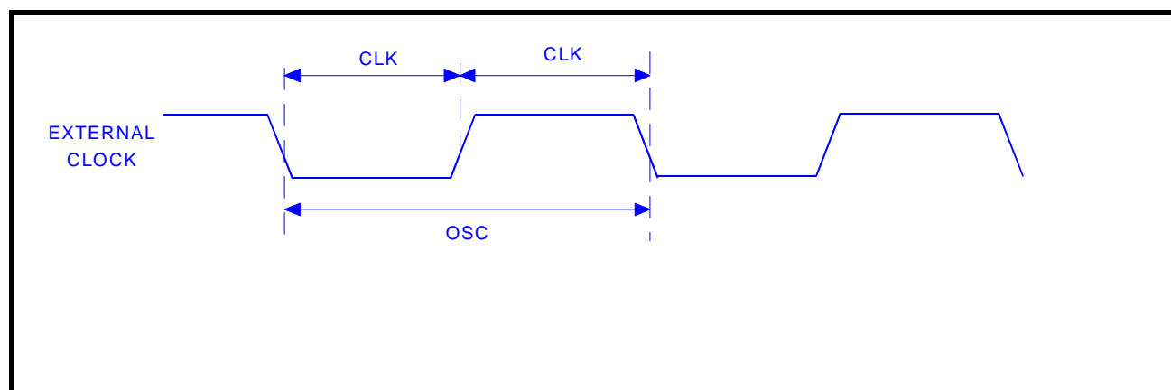
FIGURE 16. CLOCK TIMING
