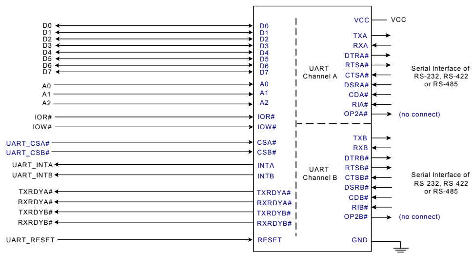
Intel Data Bus Interconnections
