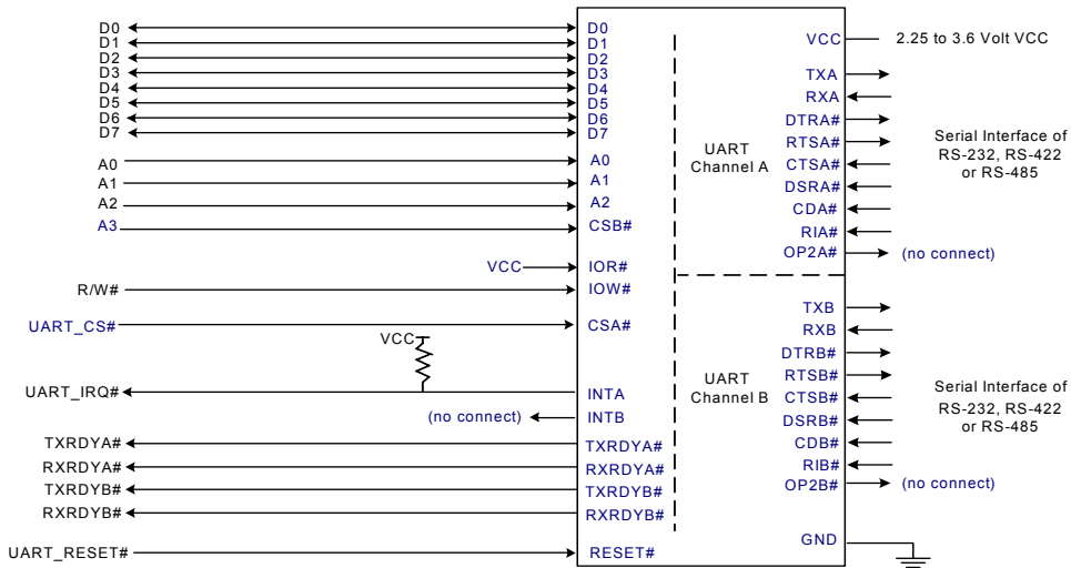
Motorola Data Bus Interconnections
