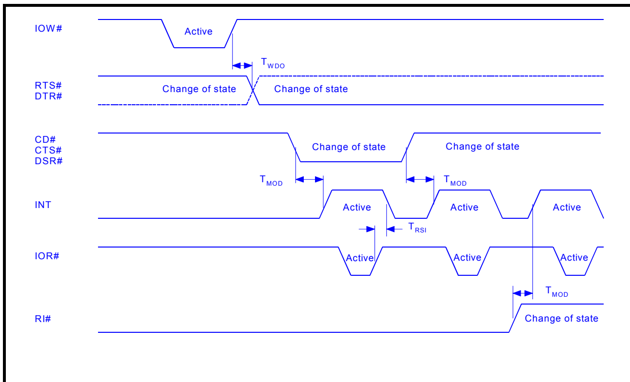
FIGURE 14. MODEM INPUT/OUTPUT TIMING FOR CHANNELS A & B
