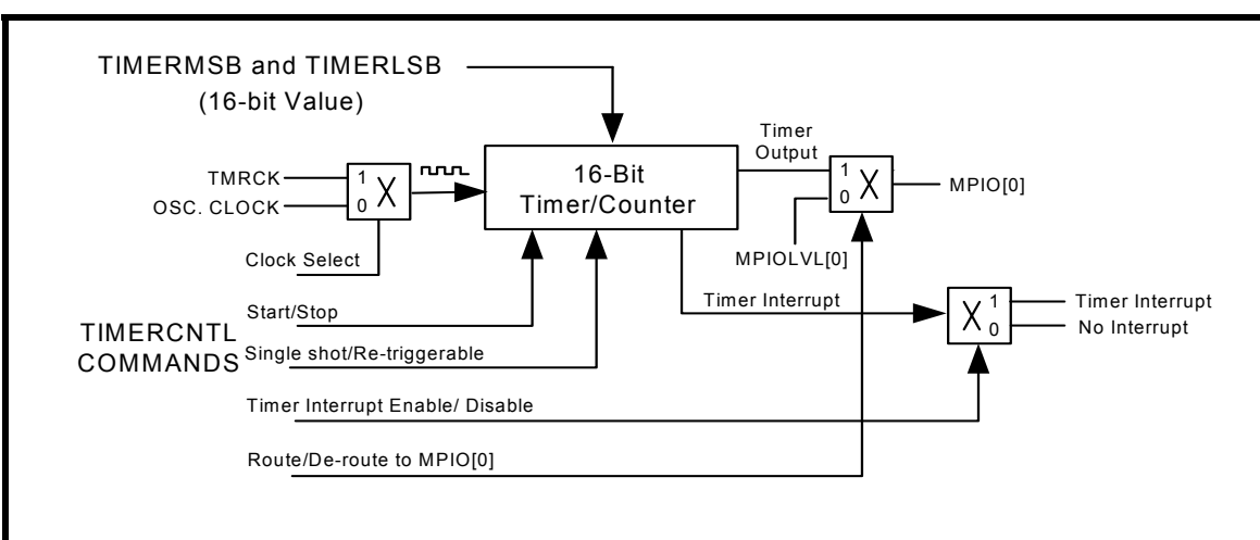
FIGURE 6. TIMER/COUNTER CIRCUIT.
