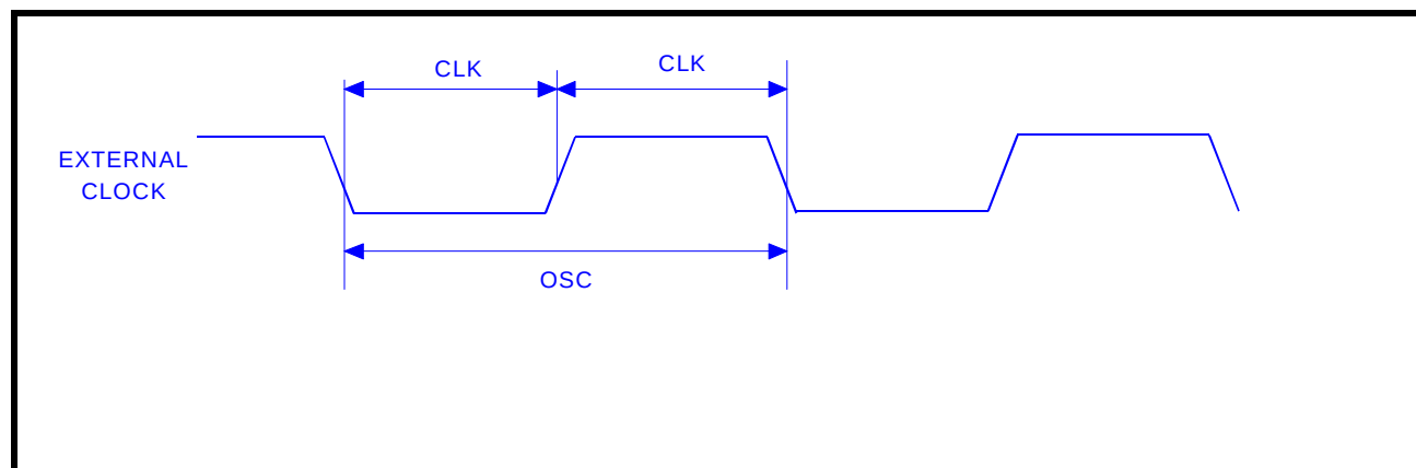
FIGURE 10. CLOCK TIMING
