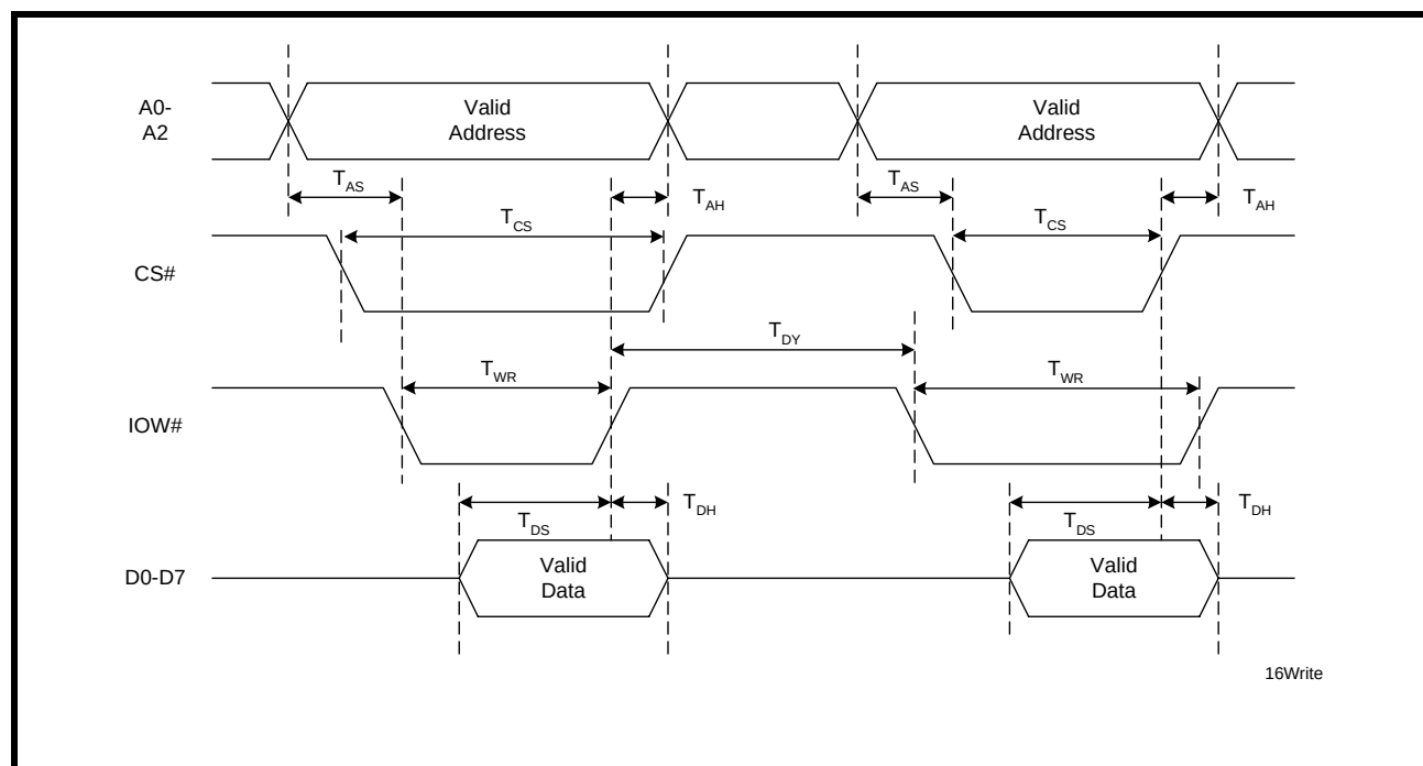
FIGURE 13. 16 MODE (INTEL) DATA BUS WRITE TIMING
