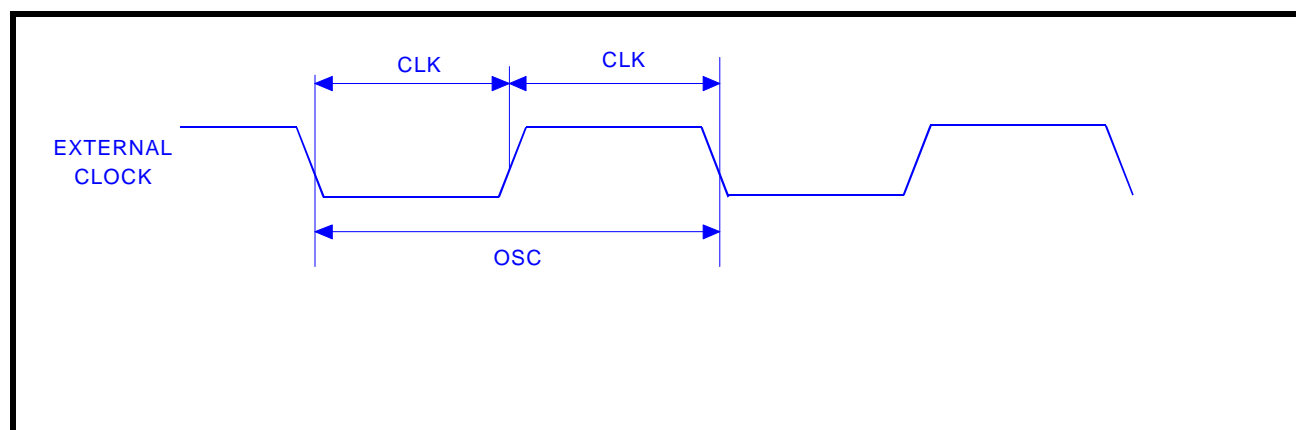
FIGURE 12. CLOCK TIMING
