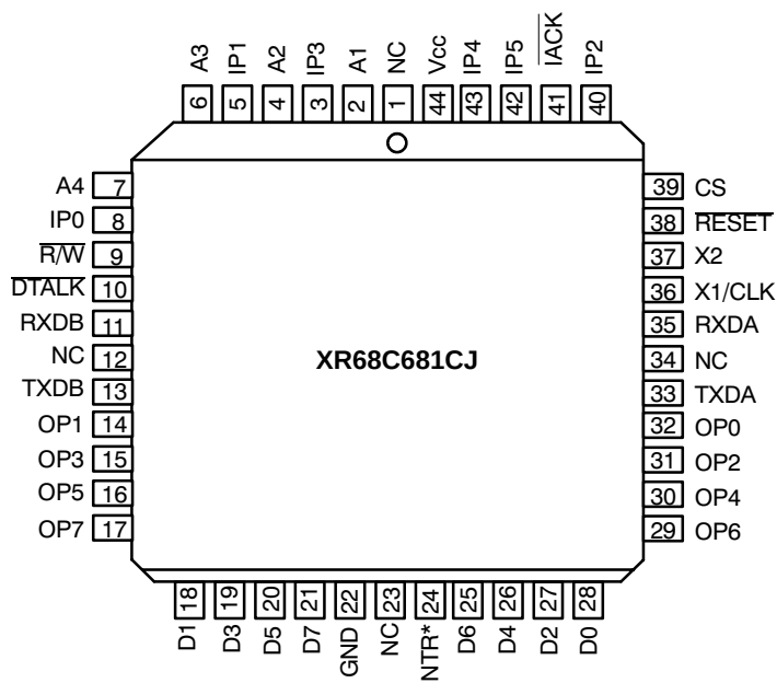
44 Pin PLCC
