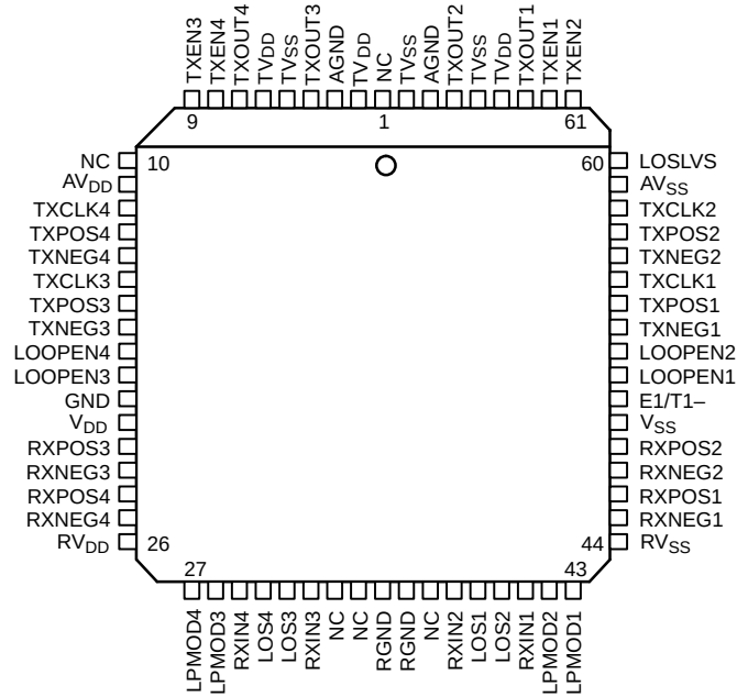
68 Lead PLCC
