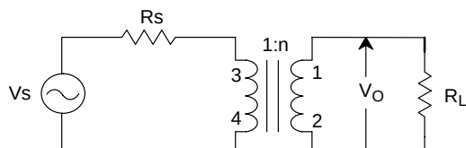
Figure 5. Equivalent Impedance Schematic
