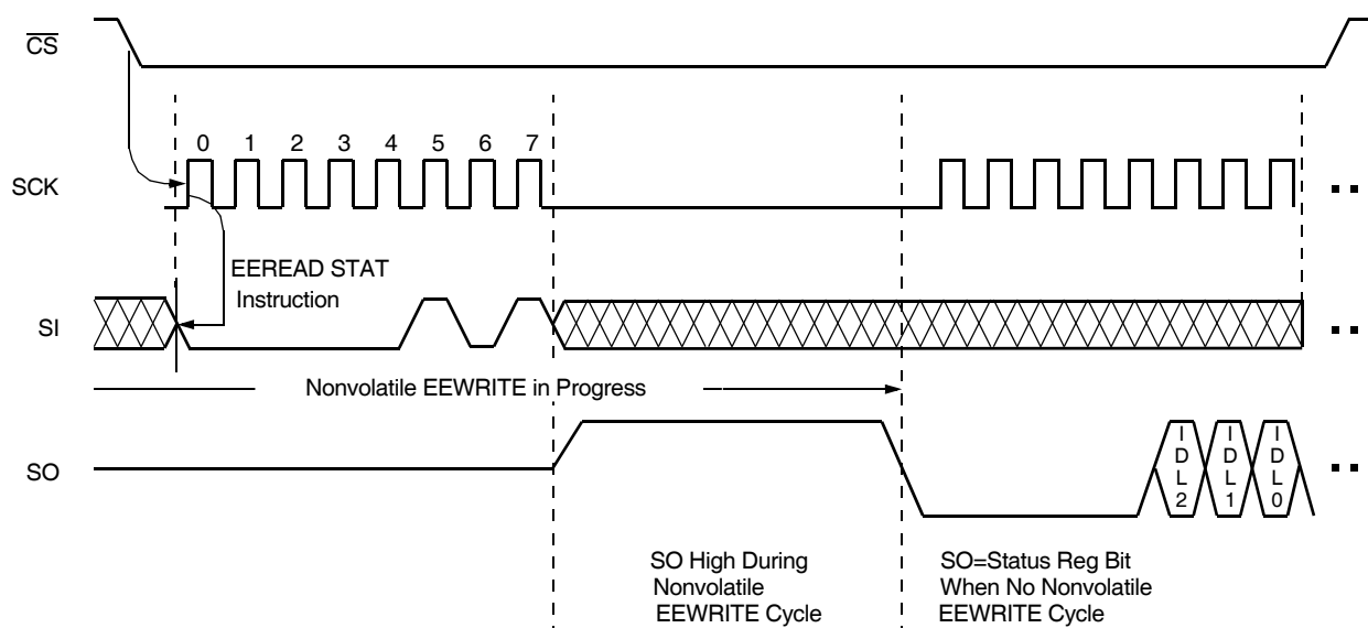
Figure 12. EEPROM Read Status (EEREAD STAT) Operation Sequence
