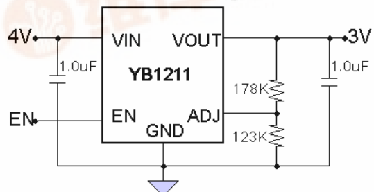
Figure 1-2 : A 3V Output Example
