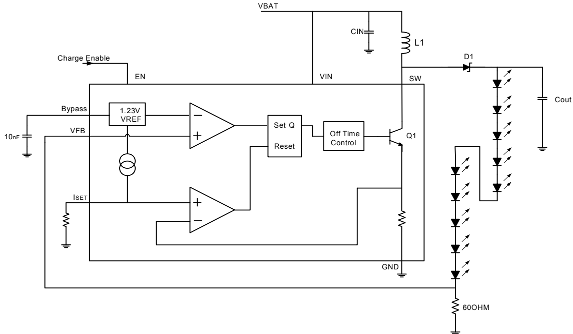
Figure 9. Block Diagram
