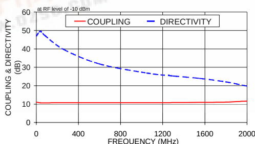
ZFDC-10-5 COUPLING & DIRECTIVITY
