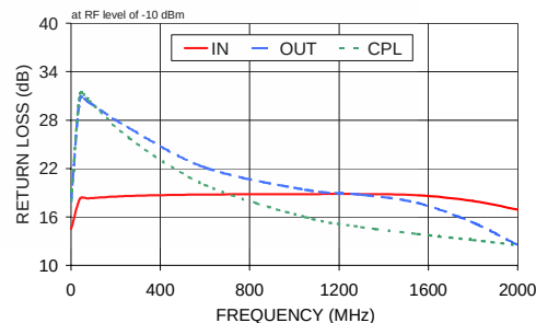
ZFDC-10-5 RETURN LOSS
