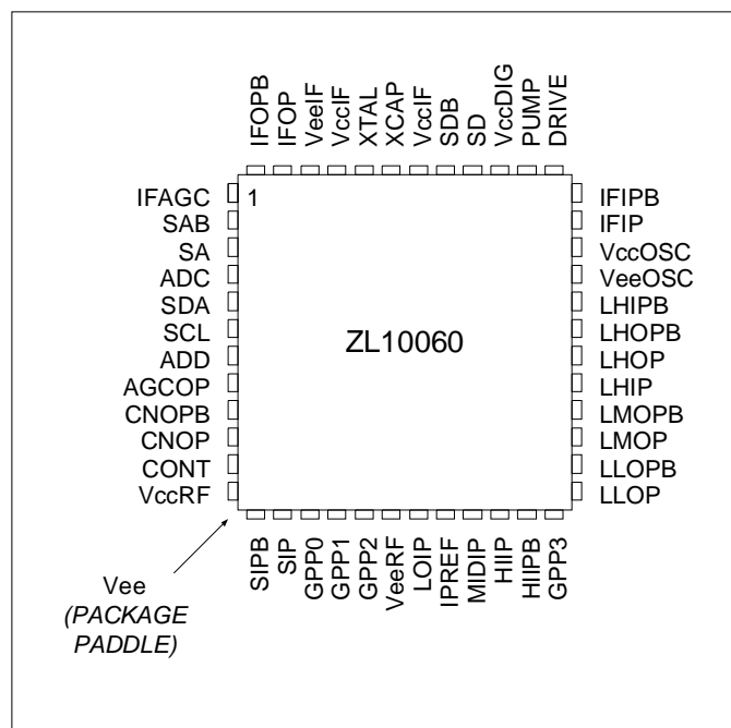
Figure 2 - Pin Diagram
