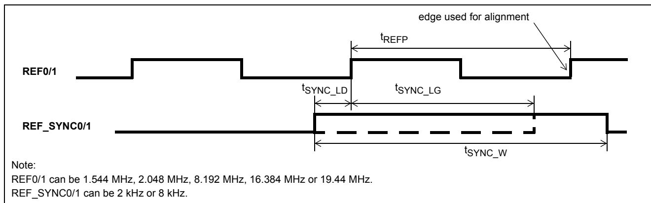
Figure 24 - REF_SYNC0/1 Timing
