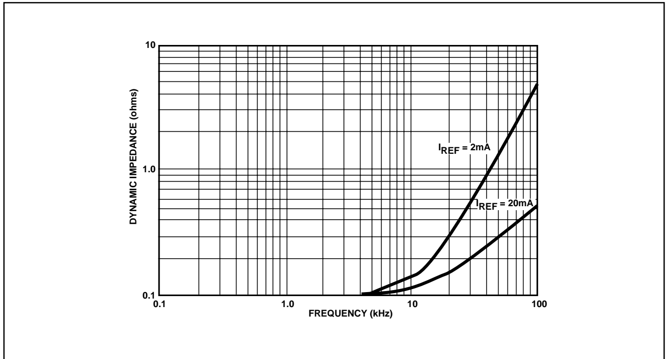
Fig.3 Dynamic impedance
