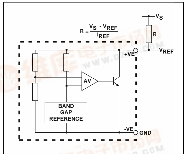
Fig.2 Circuit diagram
