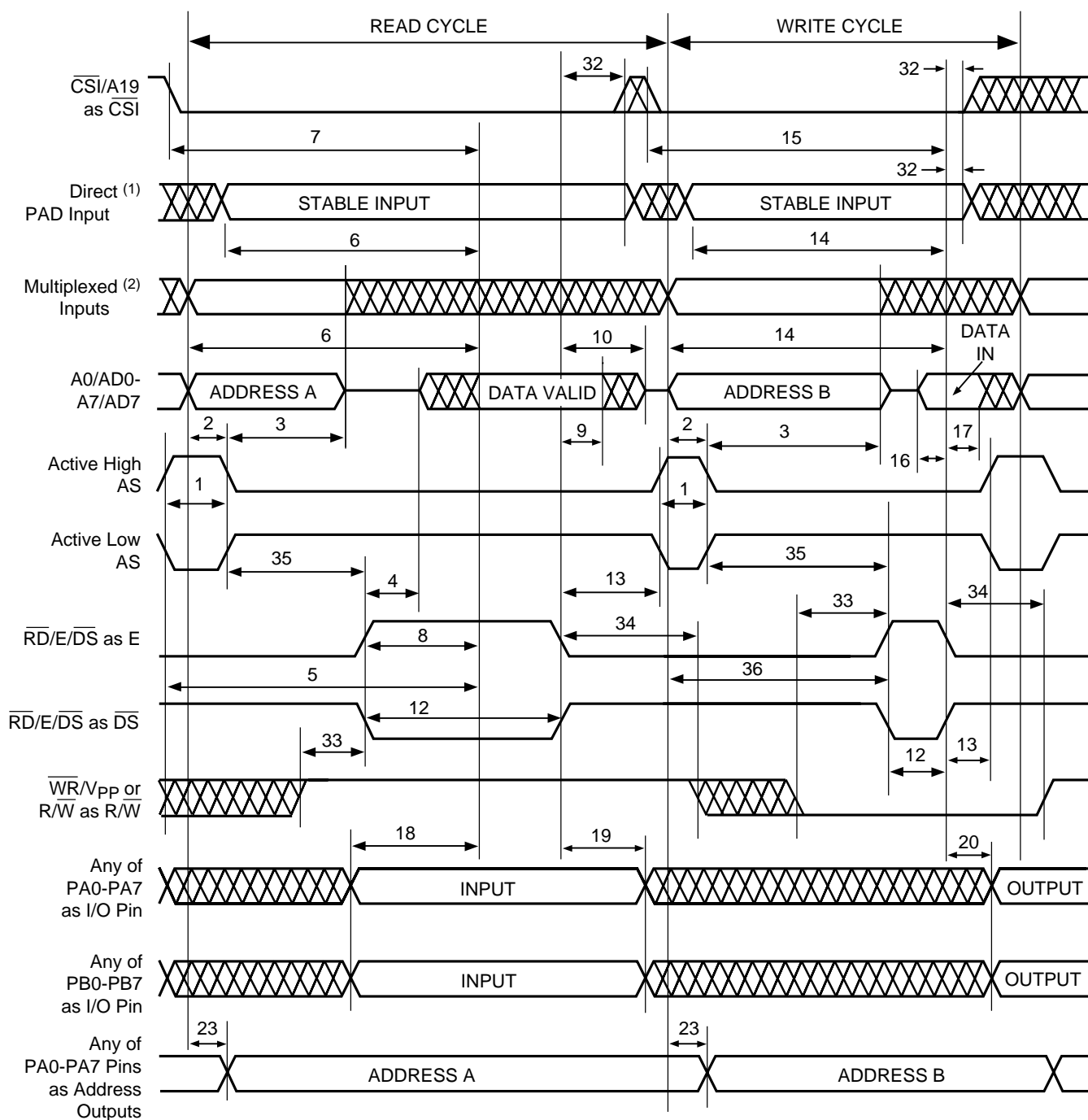
Figure 23. Timing of 8-Bit Multiplexed Address/Data Bus Using R/\bar{W} E or R/\bar{W} , \bar{D}\bar{S} (PSD3X2/3X3)
