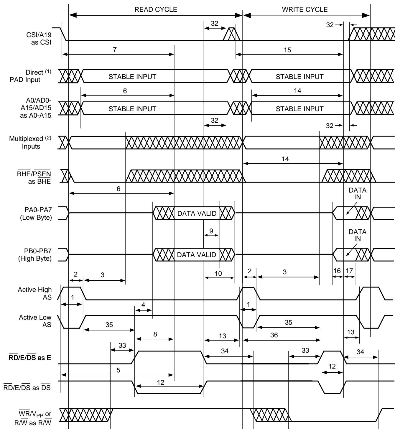
Figure 35. Timing of 16-Bit Non-Multiplexed Address/Data Bus Using R\overline{W} , E or R\overline{W} , \overline{DS} (PSD3X2/3X3)
