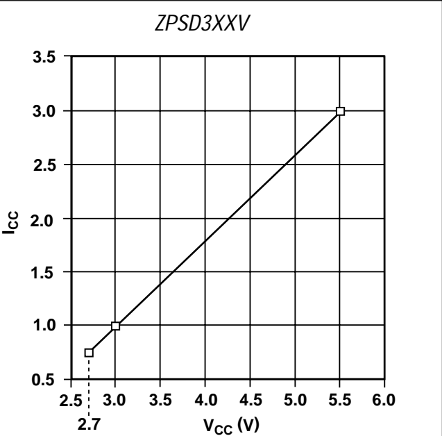
Figure 17. Normalized I_{CC} (DC vs. V_{CC} ) ( V_{CC} = 3.0\text{ V} )
