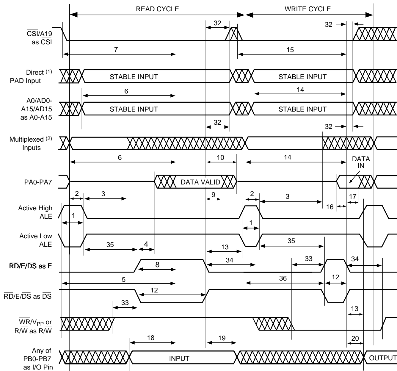
Figure 31. Timing of 8-Bit Non-Multiplexed Address/Data Bus Using R/\overline{W} , E or R/\overline{W} , \overline{DS} (PSD3X2/3X3)
