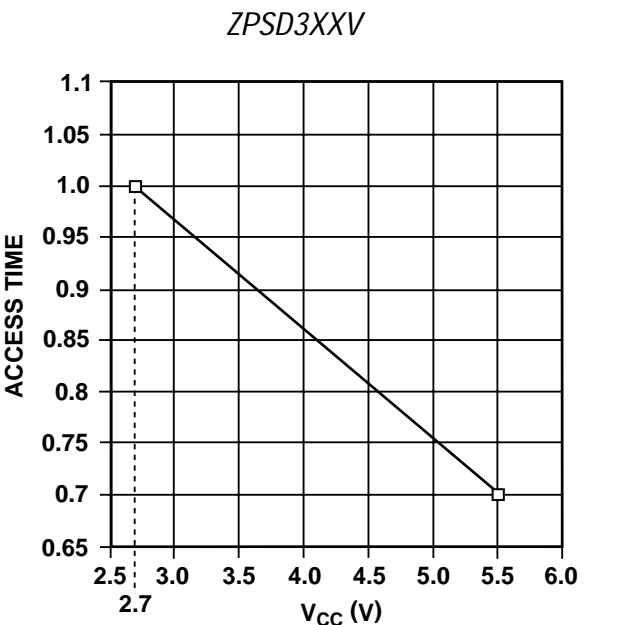
Figure 19. Normalized Access Time ( T_6 ) ( V_{CC} = 3.0\text{ V} )
