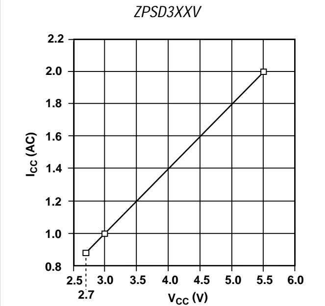
Figure 18. Normalized I_{CC} (AC) ( V_{CC} = 3.0\text{ V} )
